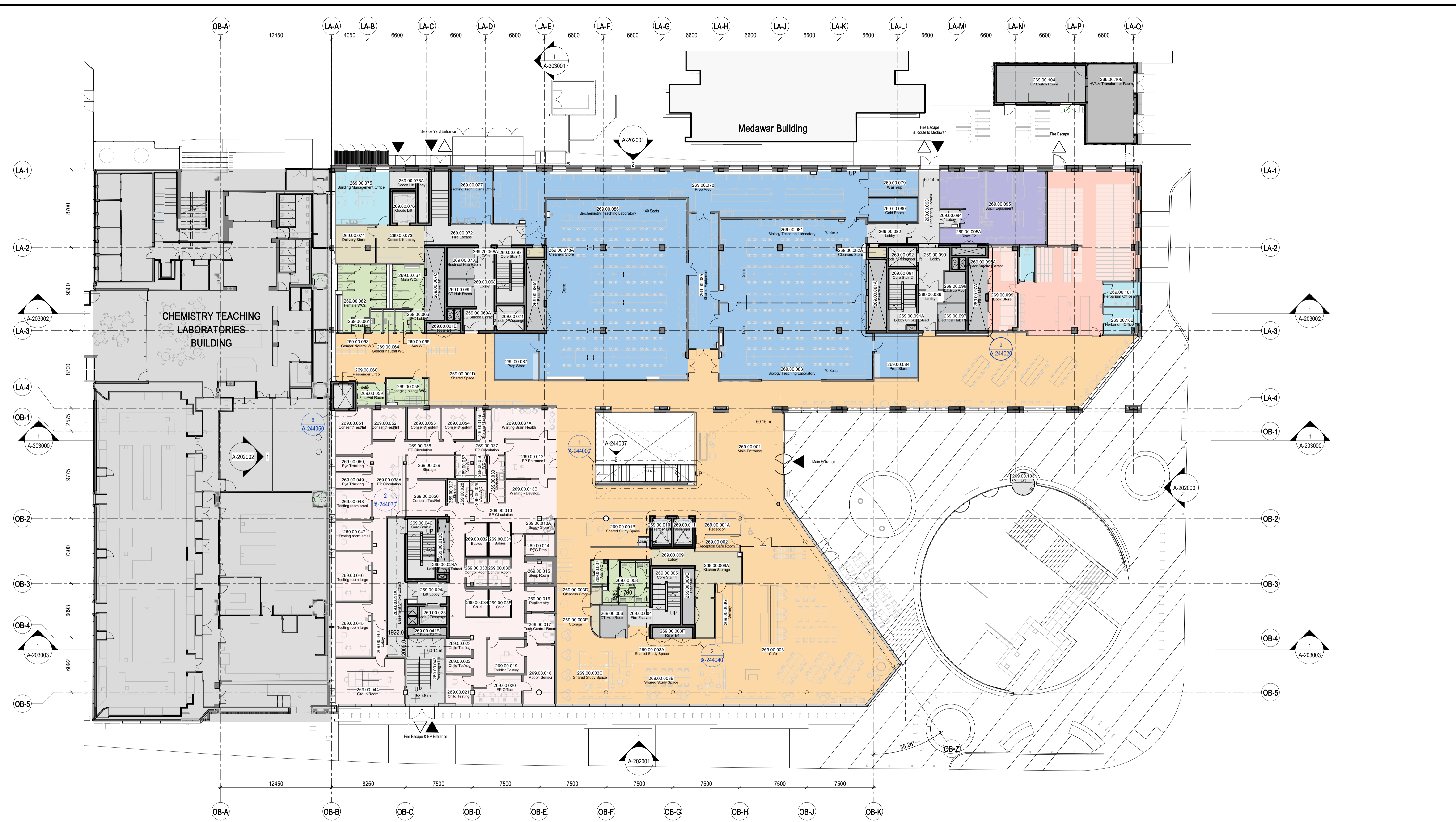
1 GROUND FLOOR PLAN 1 : 200
