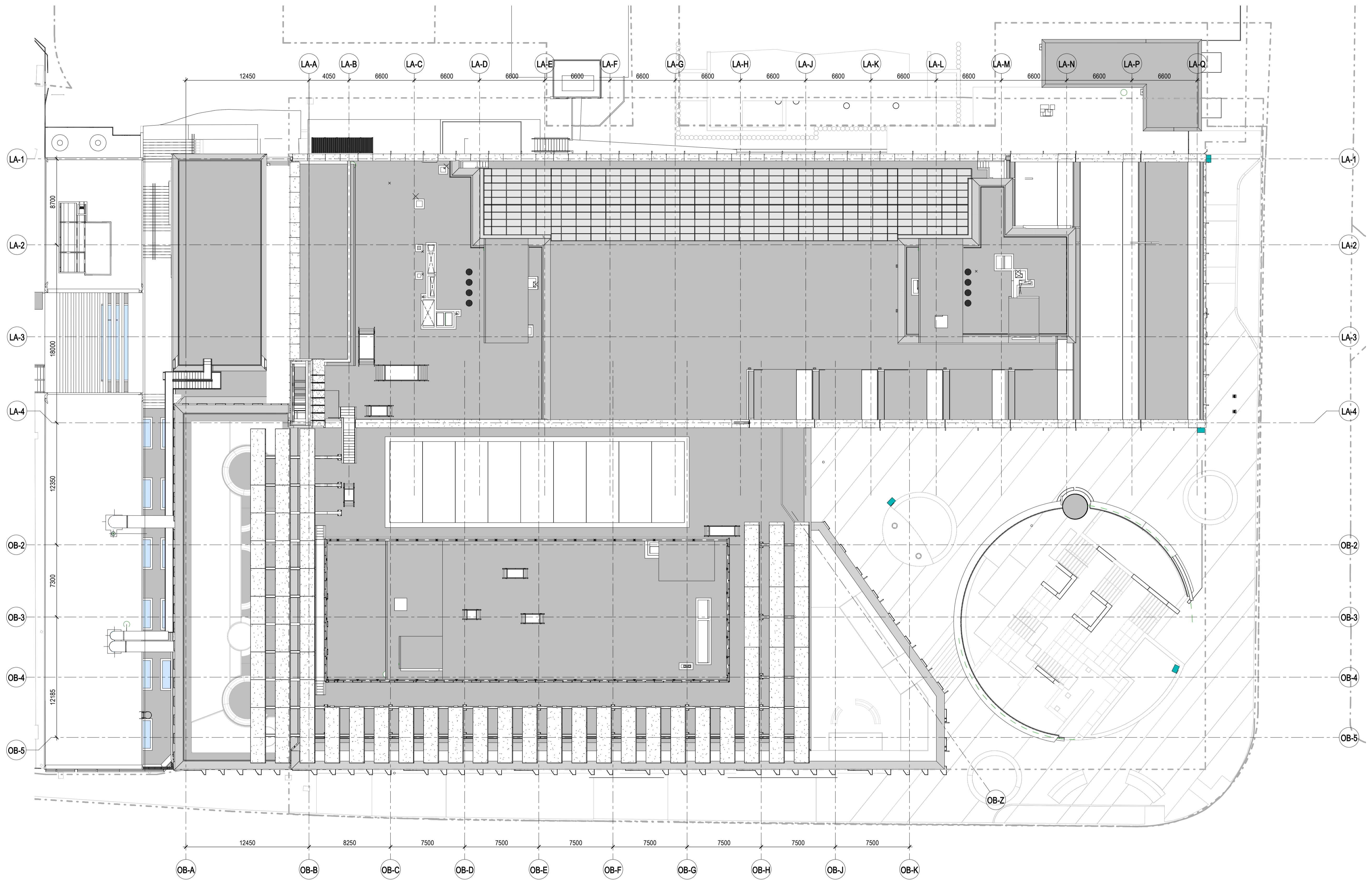
1 ROOF PLAN 1:200
